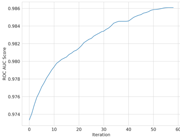
Figure 2: How AUC score varies in greedy feature selection with the addition of new features
