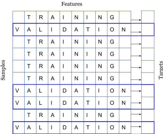
Figure 4: Splitting a dataset into training and validation sets
