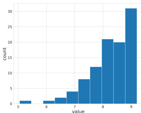
Figure 9: Histogram of f_3 after applying log transformation.
