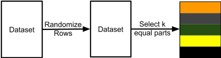
Figure 5: K-fold cross-validation
