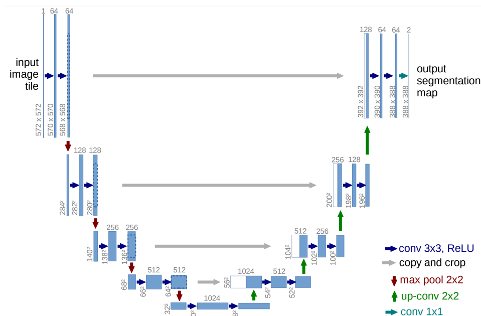
Figure 8: U-Net architecture 11 .
